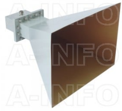
LB-770-15-C-7/16F Standard Gain Horn Antenna 0.96-1.45GHz 15dB Gain 7/16(DIN) Female
